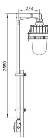
护栏式(h1) fence type
