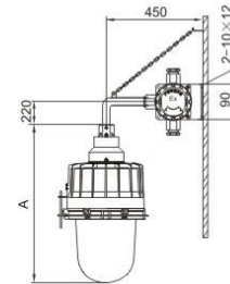
壁式(B2) Bracket type 90°
