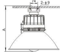
吸顶式配灯伞(X) Ceiling type With lamp umbrella
