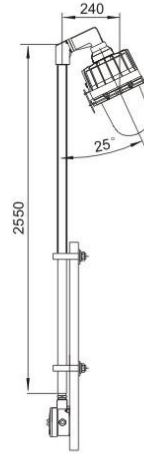
护栏式(h2) fence type
