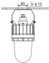
吸顶式(X) Ceiling type
